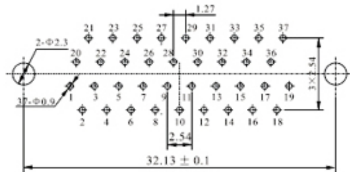
Technical drawing of a mechanical part showing dimensions: 10.6, 4.95, 2.36, 5.7, 3.7, and 3x2.54.
