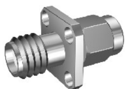
SMA-KFJ
